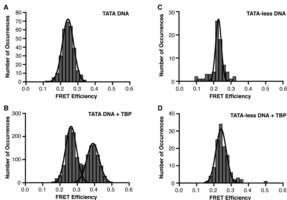
Figure 2. TBP–DNA complexes exist in a uniform FRET state. (A) Consensus TATA DNA exists in a homogeneous population in a relatively low FRET state. FRET efficiencies for 301 DNA molecules were plotted as a histogram and fit with a Gaussian. The mean FRET efficiency is 0.24. (B) In the presence of TBP, the DNA molecules exist in a two-state population (unbent and bent). Time traces for 477 DNA molecules were analyzed, and 1727 distinct FRET occurrences were plotted as a histogram and fit with Gaussians. The low and high FRET states have mean FRET efficiencies of 0.26 and 0.39, respectively. (C) Histogram and Gaussian fit of FRET efficiencies determined for 72 TATA-less DNA molecules in the absence of TBP. The mean FRET efficiency is 0.23. (D) TBP does not alter the FRET efficiency of a TATA-less DNA construct. The histogram and Gaussian fit of 124 distinct FRET occurrences observed in time traces from 121 TATA-less DNA molecules in the presence of TBP is shown. The mean FRET efficiency is 0.24.
