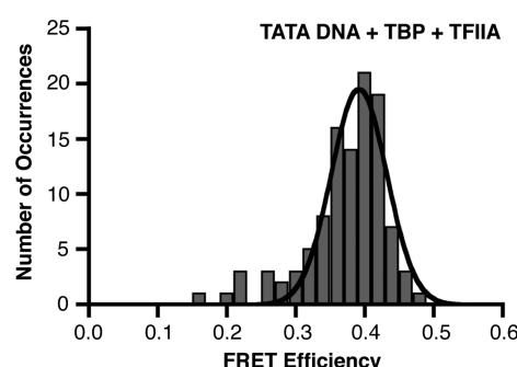
Figure 3. When included with TBP, TFIIA shifts the consensus TATA DNA to a homogeneous population in the higher FRET state. Shown is the histogram and Gaussian fit of 107 distinct FRET occurrences observed in time traces from 91 consensus DNA molecules in the presence of TBP and TFIIA; the mean FRET efficiency is 0.39.
