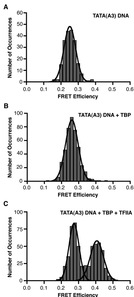
Figure 4. TFIIA facilitates the bending of the mutant TATA(A3) sequence by TBP. (A) In the absence of TBP, the mutant TATA sequence exists in a uniform FRET state similar to that observed with the consensus TATA sequence. The mean FRET efficiency for the Gaussian fit of data from 206 DNA molecules is 0.25. (B) TBP does not shift the TATA(A3) DNA into a higher FRET state. Shown is the histogram and Gaussian fit of 427 distinct FRET occurrences observed in time traces from 414 TATA(A3) DNA molecules in the presence of TBP; the mean FRET efficiency is 0.26. (C) TFIIA facilitates the bending of the TATA(A3) DNA by TBP. The mean FRET efficiencies of the low (319 occurrences) and high (274 occurrences) states obtained from the Gaussian fits of distinct FRET occurrences observed in time traces from 400 TATA(A3) molecules are 0.27 and 0.41, respectively.
