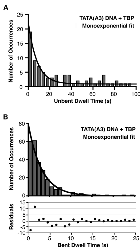
Figure 7. Unbending on the monophasic TATA(A3) DNA. (A) Analysis of the rate at which TBP bends the TATA(A3) construct. Dwell times for the unbent occurrences observed at 50 mM KCl were histogrammed and fit to a monoexponential. The observed rate constant is 0.12 \pm 0.03 \text{ s}^{-1} , where the error represents the 95% confidence interval. (B) Unbending of the TATA(A3) construct. Dwell times for the bent occurrences observed at 50 mM KCl were histogrammed and fit to a monoexponential. Residuals are plotted below the rate plot. The rate constant obtained is 0.31 \pm 0.04 \text{ s}^{-1} , where the error represents the 95% confidence interval.
