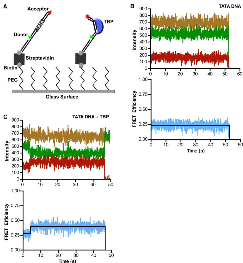
Figure 1. TBP causes an increase in the FRET observed from single immobilized consensus TATA DNA molecules. (A) Single-molecule surface configuration for monitoring TBP-induced DNA bending. When TBP bends the immobilized DNA, it causes an increase in FRET efficiency. (B) The consensus TATA construct exhibits a constant low FRET in the absence of TBP. The donor dye (green), the acceptor dye (red), and the sum of the two dyes (gold) did not change over the course of imaging (top). The calculated FRET at each time point is colored blue and the derived FRET state of 0.24 is colored black (bottom). For the purpose of display, these data were smoothed by averaging the values at three time points. (C) TBP causes an increase in FRET consistent with DNA bending. The donor and acceptor dyes show anticorrelated changes in signal intensity (top) and an increase in calculated FRET efficiency (bottom) at 4 s, indicating TBP bent the DNA. At 47 s, the acceptor dye photobleached, causing emission from the donor dye to increase. For the purpose of display, these data were smoothed by averaging the values at three time points.
