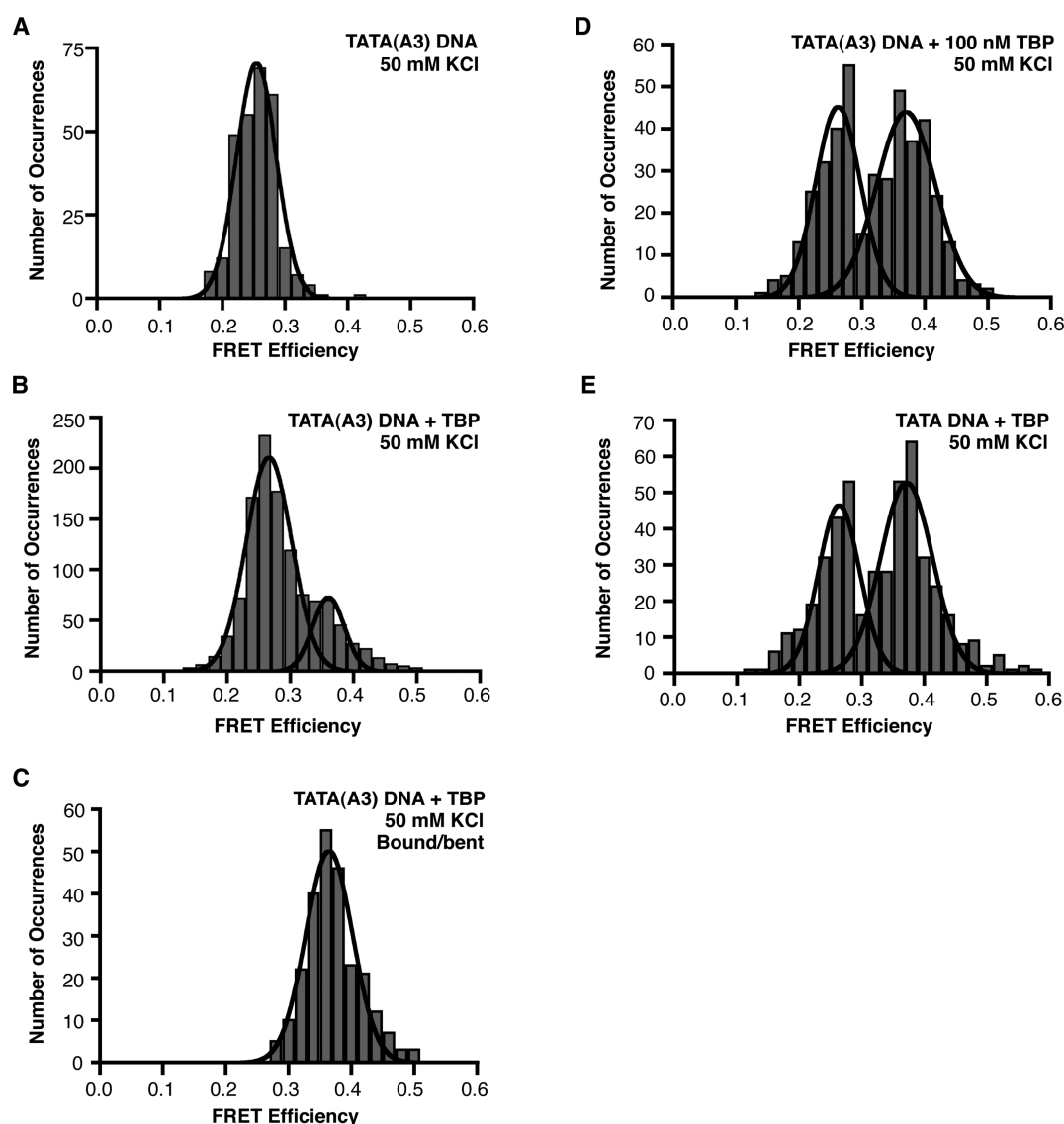
Figure 5. TBP bends the TATA(A3) sequence to a similar extent as the consensus TATA box. (A) Histogram of FRET efficiencies for 282 TATA(A3) molecules in the absence of TBP at 50 mM KCl; the mean FRET is 0.25. (B) TBP shifts a portion of the TATA(A3) DNA into a higher FRET state at 50 mM KCl; 1165 distinct FRET occurrences observed in time traces from 642 TATA(A3) molecules were histogrammed, and the low and high FRET states have mean FRET efficiencies of 0.27 and 0.36, respectively. (C) Bent states on the TATA(A3) DNA were histogrammed and fit to a single Gaussian; the mean FRET efficiency is 0.36. (D) Increasing the concentration of TBP to 100 nM increases the number of bound and bent TATA(A3) DNA molecules; 421 distinct FRET occurrences observed in time traces from 141 TATA(A3) molecules were histogrammed, and the low and high FRET states have mean FRET efficiencies of 0.26 and 0.37, respectively. (E) Bending of the consensus TATA box by TBP at 50 mM KCl. The experiment was performed with 10 nM TBP; 467 distinct FRET occurrences observed in time traces from 244 TATA molecules were histogrammed, and the low and high FRET states have mean FRET efficiencies of 0.26 and 0.37, respectively.
