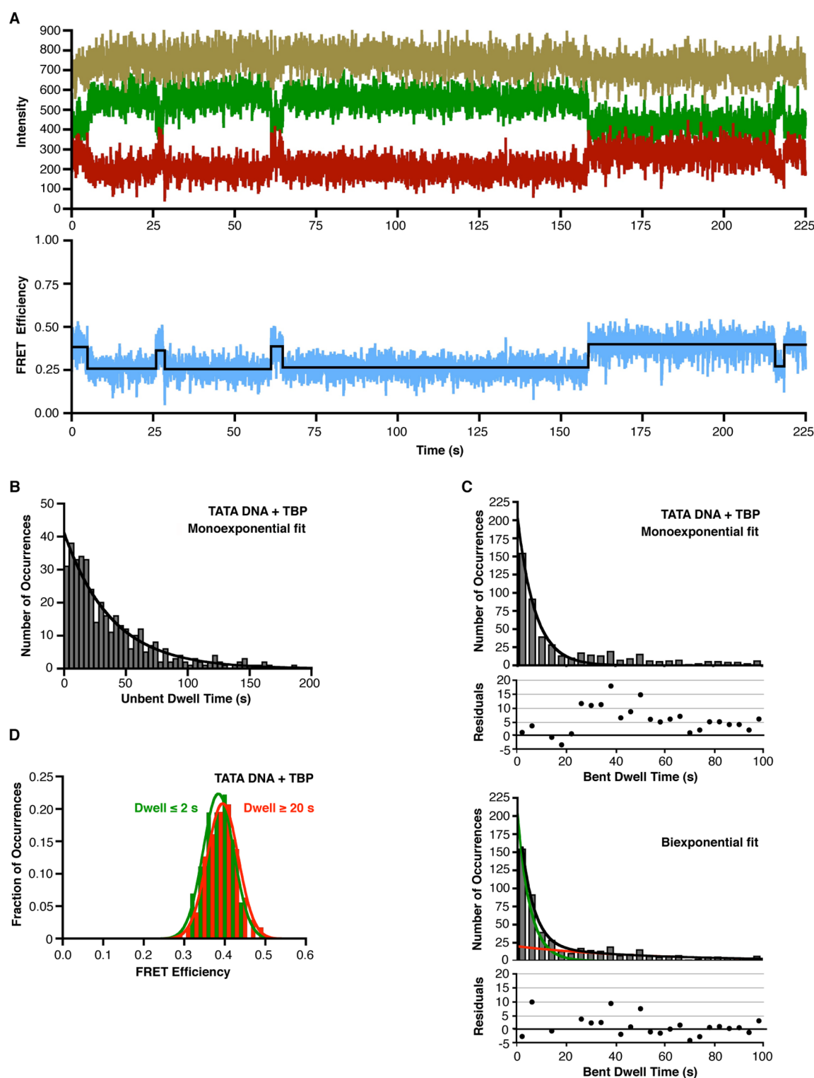
Figure 6. Unbending consensus TATA DNA is biphasic. (A) Representative time trace of a single DNA molecule switching between low FRET (unbent) and higher FRET (bent) states. The top plot shows the donor emission (green), the acceptor emission (red), and the sum of the donor and acceptor emission (gold). The bottom plot shows the corresponding FRET (blue); the black line indicates the FRET state fit of the data. For the purpose of display, these data were smoothed by averaging the values at three time points. (B) Analysis of the rate at which TBP bends the consensus TATA box. Dwell times for the unbent occurrences observed at 150 mM KCl were histogrammed and fit to a monoexponential. The observed rate constant is 0.026 \pm 0.003 \text{ s}^{-1} , where the error represents the 95% confidence interval. (C) Unbending of the consensus TATA box occurs in two distinct kinetic phases. Dwell times for the bent occurrences observed at 150 mM KCl were histogrammed and fit to a monoexponential (top) or biexponential (bottom). Residuals are plotted for each of the fits. The two rate constants obtained from the biexponential fit are 0.19 \pm 0.03 and 0.019 \pm 0.008 \text{ s}^{-1} , where the error represents the 95% confidence interval. (D) TATA DNA molecules in complexes with different kinetic stabilities are bent to the same extent. FRET efficiencies were separately histogrammed for bent occurrences having dwell times of \leq 2 s (green) or \geq 20 s (red). Gaussian fits showed mean FRET efficiencies of 0.38 and 0.39, respectively.
